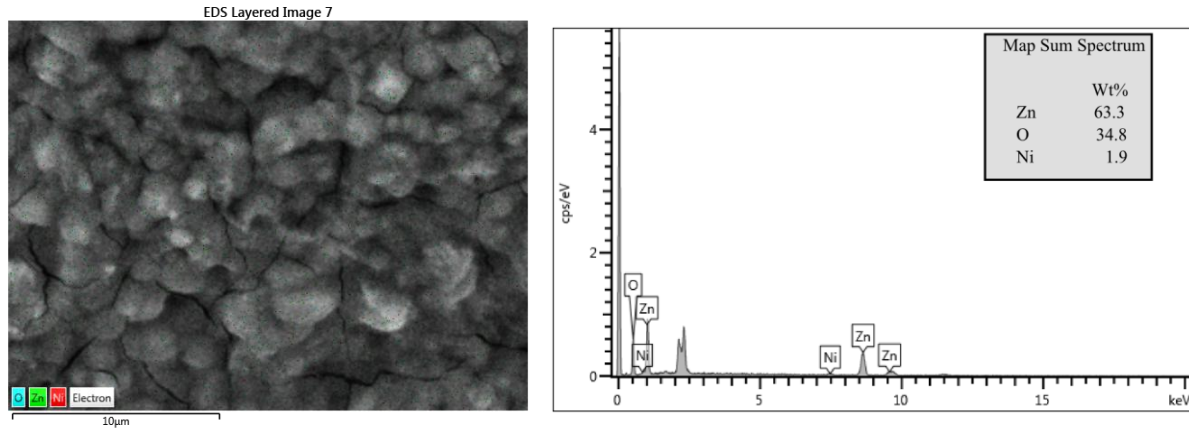
Figure 3: SEM images and EDS results on the nanoparticles with 4 wt.% Ni-ZnO
